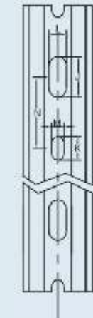
Single mounting pattern up to 60mm width
