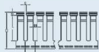
Single Restricted slot up to 50mm Height
