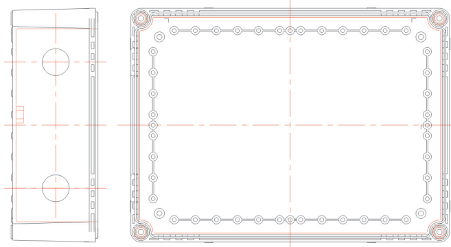
Tailor drilled cable gland holes (Article No. 01 17 00228)
