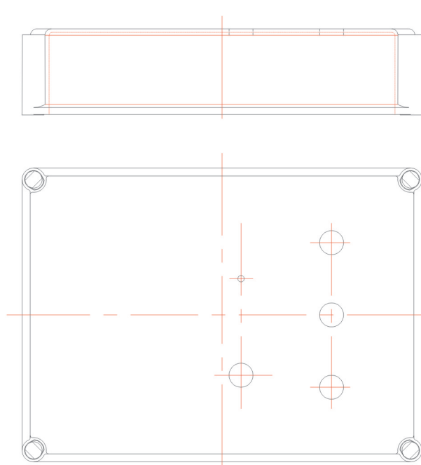
Tailor drilled push button holes (Article No. 01 17 00227)
