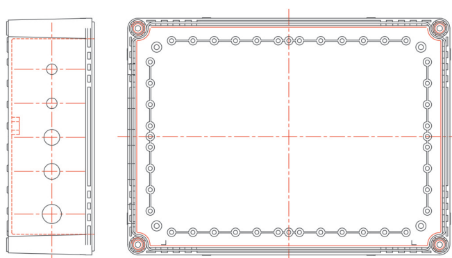
Tailor drilled cable gland holes (Article No. 01 17 00289)
