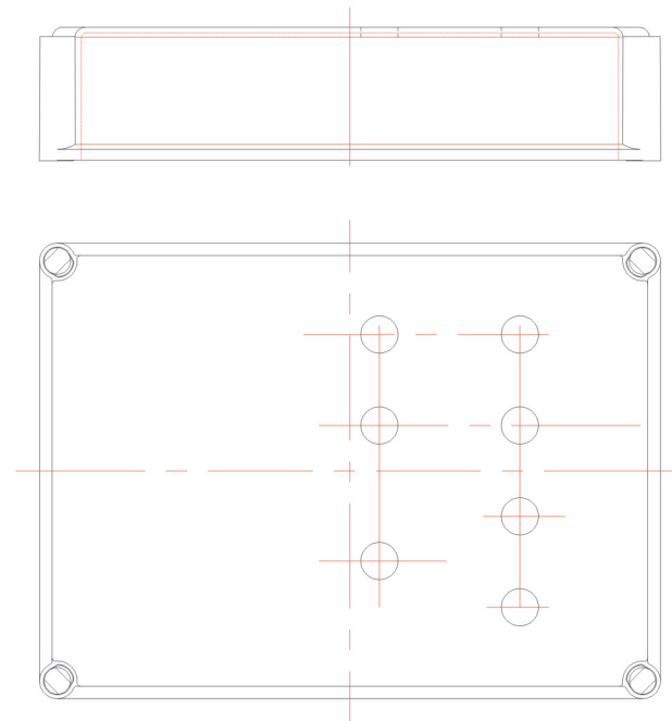
Tailor drilled push button holes (Article No. 01 17 00226)
