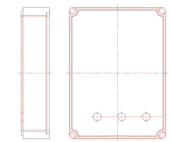
Tailor drilled push button holes (Article No. 01 17 00227)
